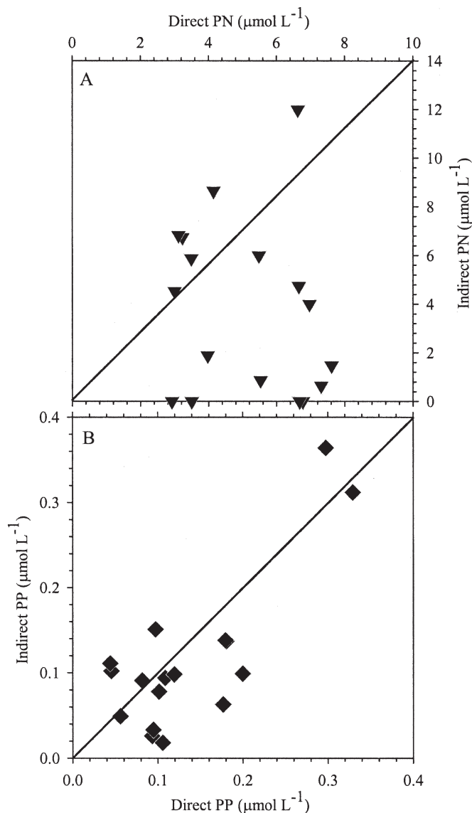
Fig. 7. (A) Particulate nitrogen (PN) and (B) particulate phosphorus (PP) concentrations estimated by direct versus indirect measurement. Each symbol is a location (2 per site; Lox8, F1, F4, and U3) or depth (3 per site; 3A5 Cladium, 3A5 Slough, and SrsA) from sites across the Everglades.
