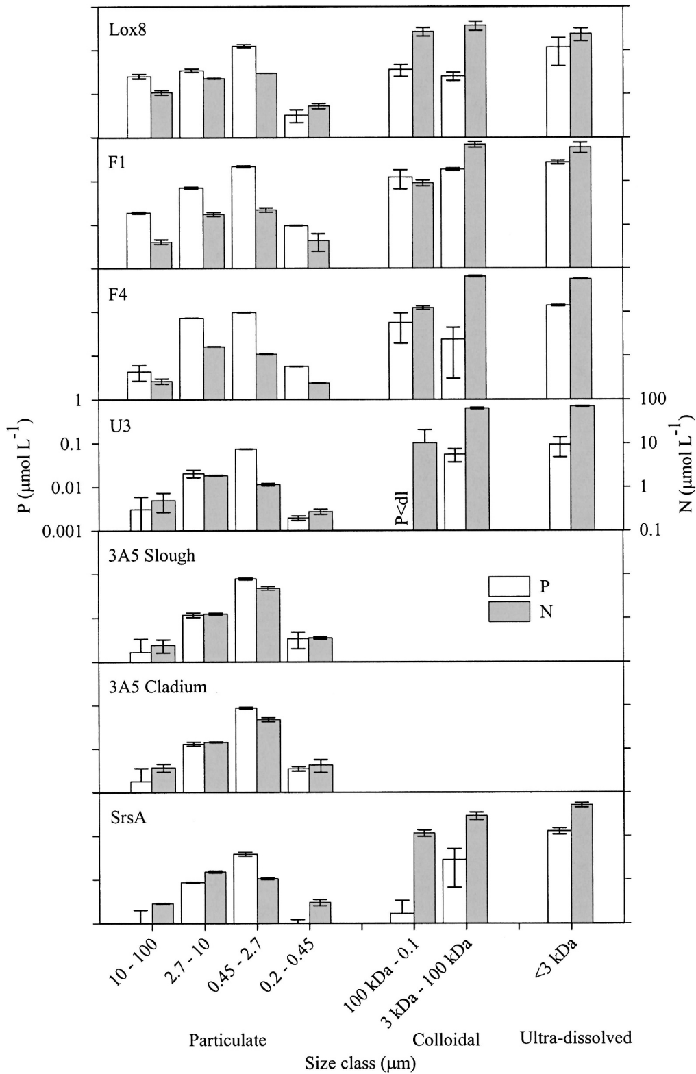
Fig. 3. Phosphorus and nitrogen concentrations in particulate (left bars, \mu\text{m} ), colloidal (center bars, \mu\text{m} to kDa), and ultrafiltered dissolved (right bars, kDa) size classes at sites across the Everglades. Colloidal size classes were not sampled at 3A5 Slough and 3A5 Cladium sites. P<dl = phosphorus below detection limit. Mean \pm one SE; n = 2 locations (Lox8, F1, F4, and U3) or 3 depths (3A5 Cladium, 3A5 Slough, and SrsA).
