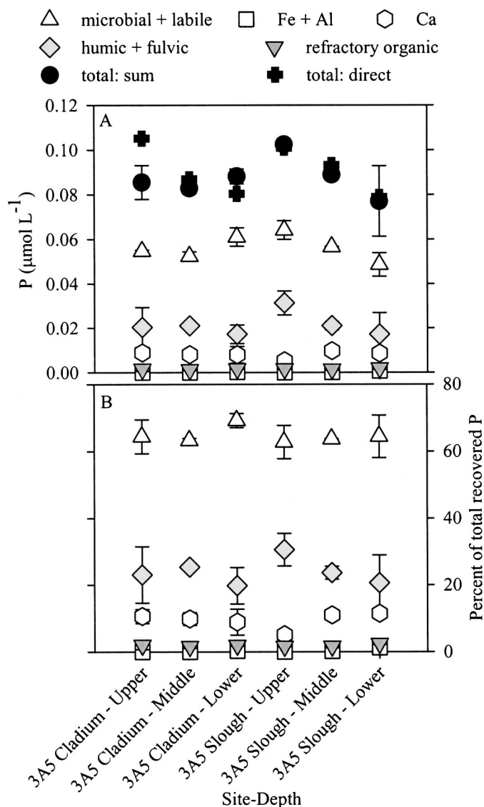
Fig. 6. Sequential chemical extraction of particulate phosphorus in the upper, middle, and lower water column of the 3A5 Cladium and 3A5 Slough sites. (A) Concentrations and (B) percent of total recovered P are shown for each form of P associated with the sequential chemical extraction of suspended particles. Total phosphorus concentrations are presented as the sum of the individual extractions and the sum of total particulate phosphorus collected on different filters and measured directly. Mean \pm one SE; n = 2 .
