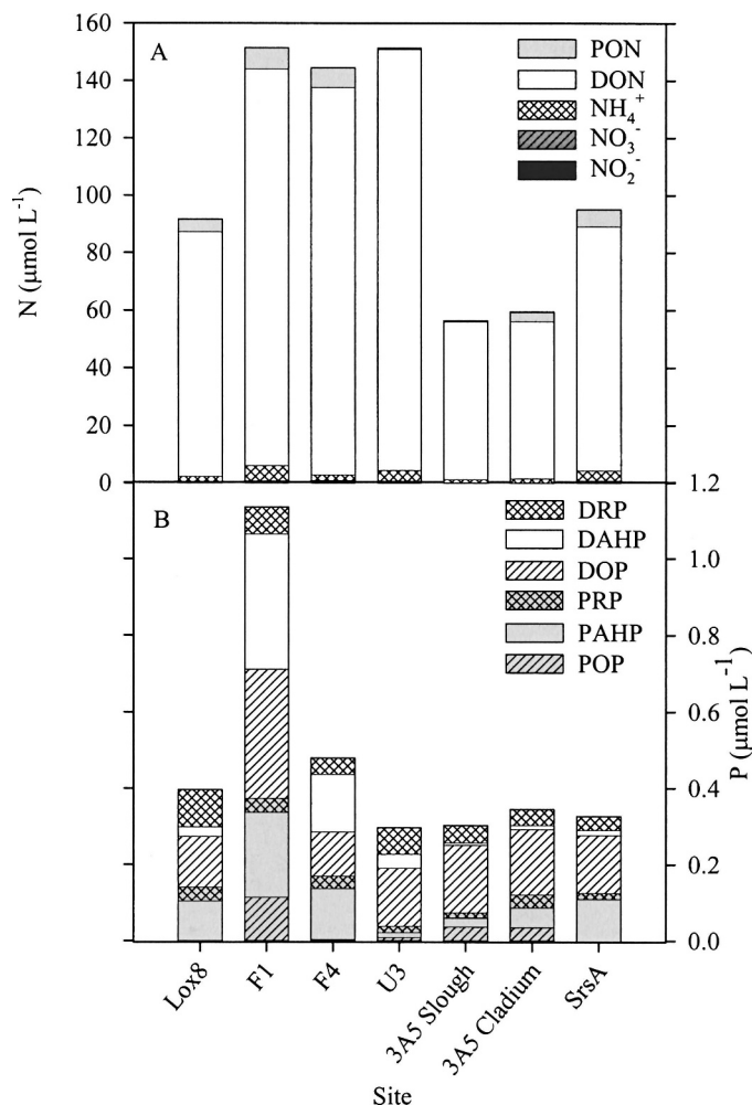
Fig. 5. (A) Speciation of dissolved ( <0.2 \mu\text{m} ) and particulate ( >0.2 \mu\text{m} ) nitrogen and (B) phosphorus at sites across the Everglades. DON = dissolved organic nitrogen, PON = particulate organic nitrogen, POP = particulate organic phosphorus, PAHP = particulate acid-hydrolyzable phosphorus, PRP = particulate reactive phosphorus, DOP = dissolved organic phosphorus, DAHP = dissolved acid-hydrolyzable phosphorus, DRP = dissolved reactive phosphorus. Mean; n = 2 locations (Lox8, F1, F4, and U3) or 3 depths (3A5 Cladium, 3A5 Slough, and SrsA).
