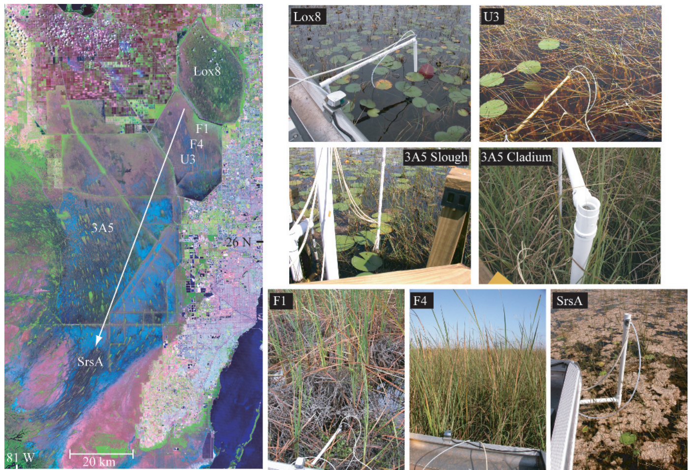
Fig. 1. False-color satellite image of the Everglades and south Florida showing the locations of the sampling sites and individual photos of each sampling site. Generalized flow direction is shown as an arrow on the satellite image. See Table 1 for the site labels.
