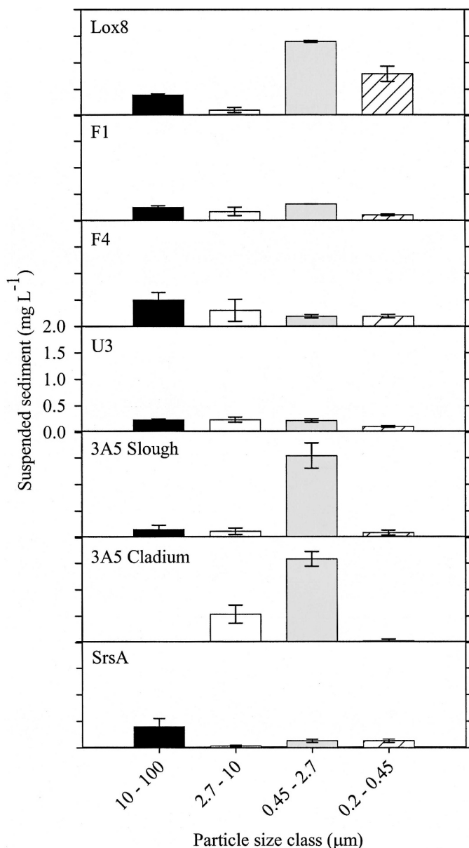
Fig. 2. Suspended sediment concentrations in each size class at sites across the Everglades. Mean \pm one SE; n = 2 locations (Lox8, F1, F4, and U3) or 3 depths (3A5 Cladium, 3A5 Slough, and SrsA).
