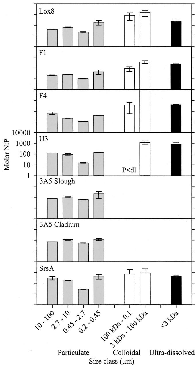
Fig. 4. Nitrogen : phosphorus molar ratio in particulate (left bars, \mu\text{m} ), colloidal (center bars, \mu\text{m} to kDa), and ultrafiltered dissolved (right bars, kDa) size classes at sites across the Everglades. Colloidal size classes were not sampled at 3A5 Slough and 3A5 Cladium sites. P < \text{dl} = phosphorus below detection limit. Mean \pm one SE; n = 2 locations (Lox8, F1, F4, and U3) or 3 depths (3A5 Cladium, 3A5 Slough, and SrsA).
